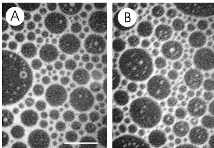
FIGURE 3 Visualization of laterally condensed domains in binary monolayers of 16:0-DHSM (A) and 16:0-SM (B) and cholesterol. The monolayers of the sphingomyelins were prepared to include 30 mol % cholesterol together with 1.0 mol % NBD-cholesterol. The monolayers were compressed at a speed not exceeding 5 \text{ \AA}^2/\text{molecule}/\text{min} . The lateral domains were documented at a lateral surface pressure of 1 \text{ mN/m} during the first compression. Scale bar, 50 \text{ }\mu\text{m} .
